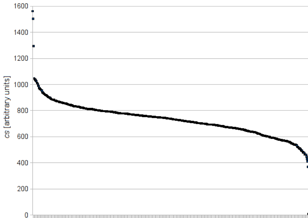
Fig. 2. – Experiment 1: Cumulative similarity cs of the worst gene for each miRNA w.r.t. all the remaining ones, as a measure of its likelihood to be recognized as match – sorted in decreasing order along the horizontal axis.
